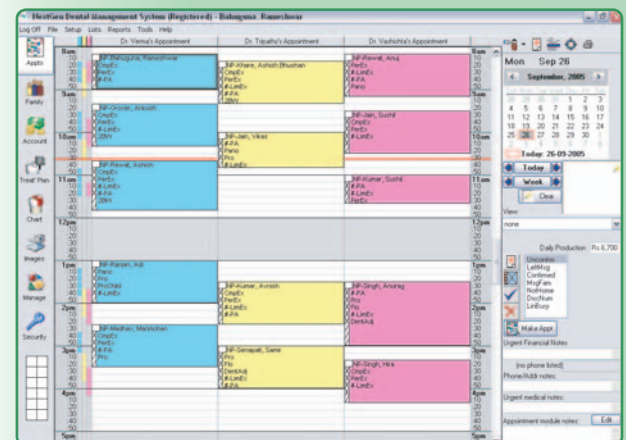
Appointment Module
